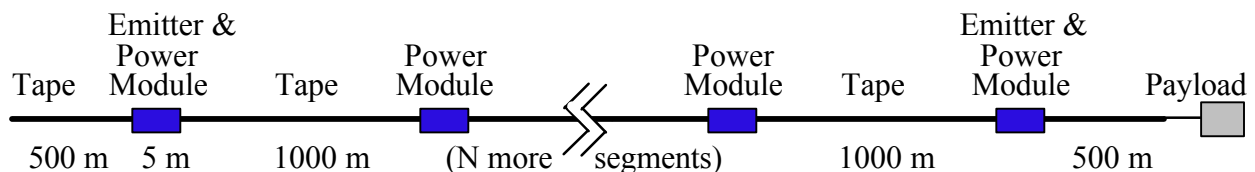
Figure 4. Schematic of Operational Version of EDDE
