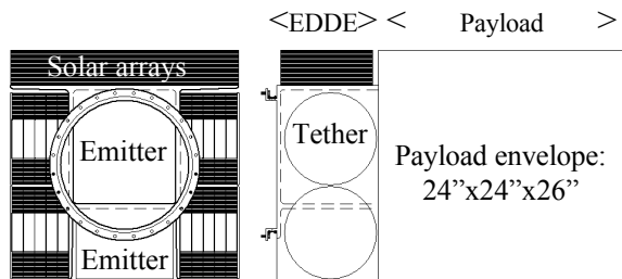
Radial view from ESPA Tangential view with payload
