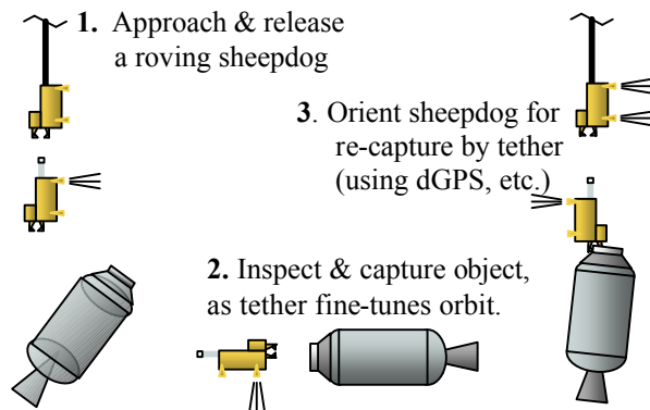
Figure 12. “Sheepdogs” for Two-Stage Capture
